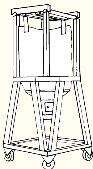
MOBILE BAGSTANDER
